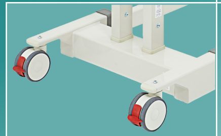
Concealed Electric Leg Spread Mechanism
